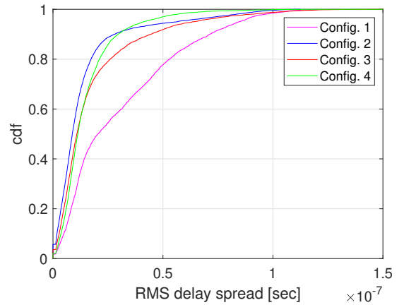
Fig. 10. CDF of the RMS delay spread for the four AP configurations
