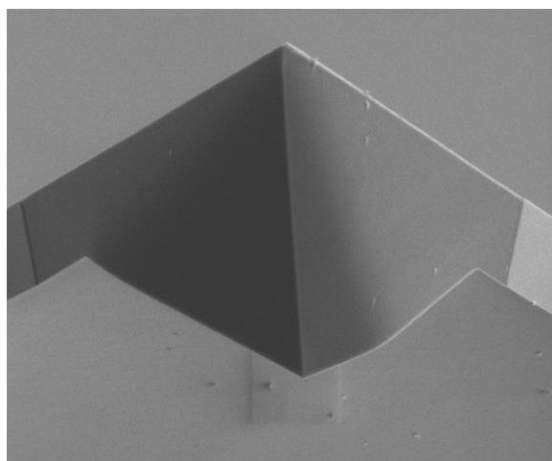
View of a first generation tip probe for IR and THz frequencies (made in July 2014)
